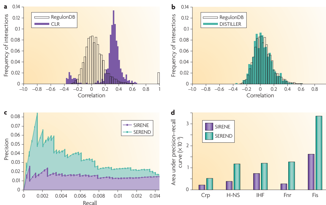
Figure 3 | The different characteristics of interactions inferred by expression-based and integrative network inference methods.
