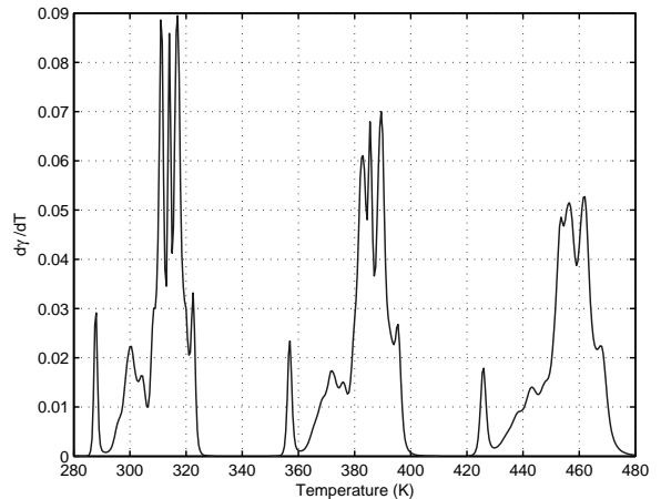
FIG. 6: PN/MCS13 Differential melting curves for \Gamma = -0.05 , 0.0 , and 0.05 eV/rad (left to right, temperature increment 0.5 K ).
