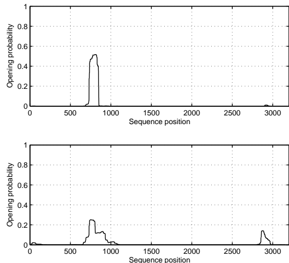
FIG. 11: Opening probability at T = 310 K in fixed torque ensemble for the C-MYC sequence ( N = 3200 , \Gamma = -0.041475 , \langle \sigma \rangle_\Gamma = -0.03004 ) (top) and the modified C-MYC sequence ( N = 3156 , \Gamma = -0.044365 , \langle \sigma \rangle_\Gamma = -0.03003 ) (bottom).
