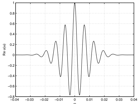
FIG. 9: C-MYC Real value of u(\omega) (eq. (12)) at \sigma = -0.03 ( \alpha = 0.59 ) and T = 310 K ( \omega -interval 5 \cdot 10^{-4} ).
