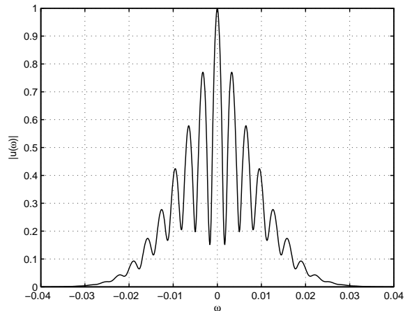
FIG. 8: C-MYC Absolute value of u(\omega) (eq. (12)) at \sigma = -0.03 ( \alpha = 0.59 ) and T = 310 K ( \omega -interval 5 \cdot 10^{-4} ).
