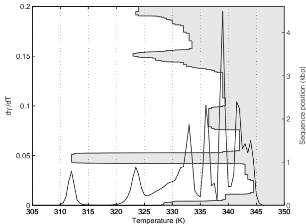
FIG. 4: PN/MCS13 Differential melting curve and melting map (shaded area) with homogeneous stacking and twist energy ( K = 0.1486 eV , E = 0.0942 eV , \theta_0 = 34.81^\circ ) (temperature increment 0.5 K , \Gamma = -0.042 eV/rad ).
