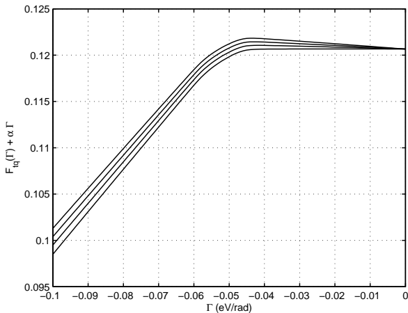
FIG. 7: C-MYC F_{tq}(\Gamma) + \alpha\Gamma for \alpha = 0.572, 0.581, 0.590, 0.600 (top to bottom) at T = 310 K .
