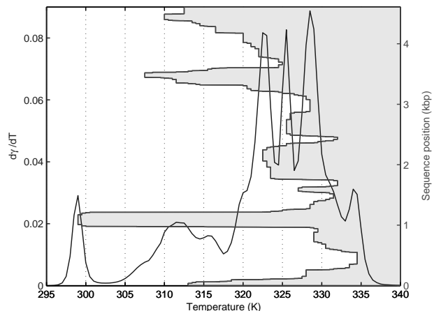
FIG. 3: PN/MCS13 Differential melting curve and melting map (shaded area) (temperature increment 0.5 K, \Gamma = -0.042 eV/rad).
