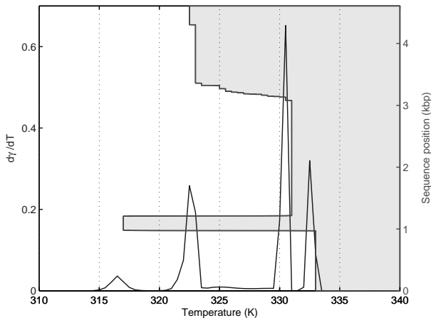
FIG. 5: PN/MCS13 Differential melting curve and melting map (shaded area) with homogeneous stacking and twist energy ( K = 0.65 eV , E = 0.04 eV , \theta_0 = 34.78^\circ ) (temperature increment 0.5 K , \Gamma = -0.042 eV/rad ).
