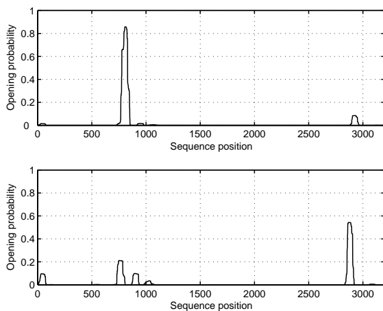
FIG. 10: Opening probability at T = 310 K and fixed superhelical density \sigma = -0.03 for the C-MYC sequence ( N = 3200 ) (top) and the modified C-MYC sequence ( N = 3156 ) (bottom).
